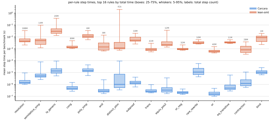
Fig. 4. Mean time per step of each rule, over the benchmarks whose elaborated proof both checkers accept, for the sixteen rules with the largest total time, pooling the two solvers. The two series share an x position. Boxes are the quartiles and whiskers the 5th and 95th percentiles; the label above each group is the rule’s total step count in the round. Note the log scale: CARCARA sits three to four decades below LEAN-SMT throughout.
