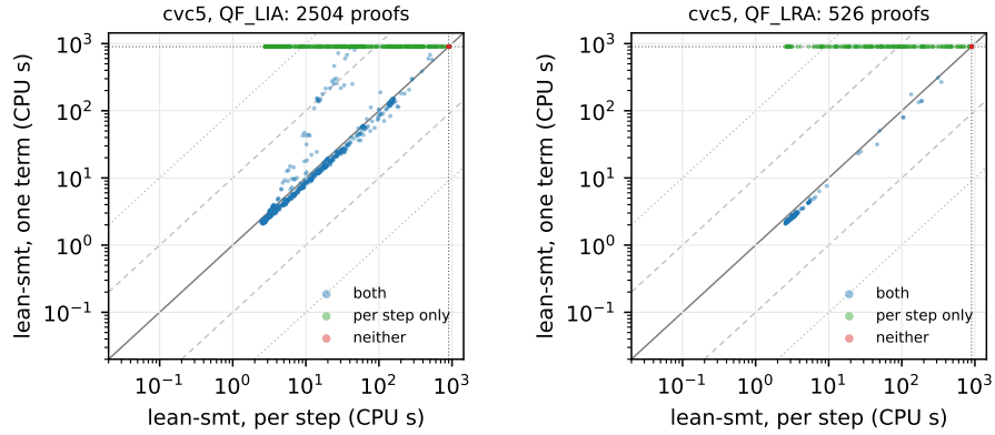
Fig. 8. The same comparison on cvc5's arithmetic proofs, QF_LIA (left) and QF_LRA (right). The proofs are smaller, so both shapes reach further, and the one-term shape still loses 812 and 217 benchmarks.
