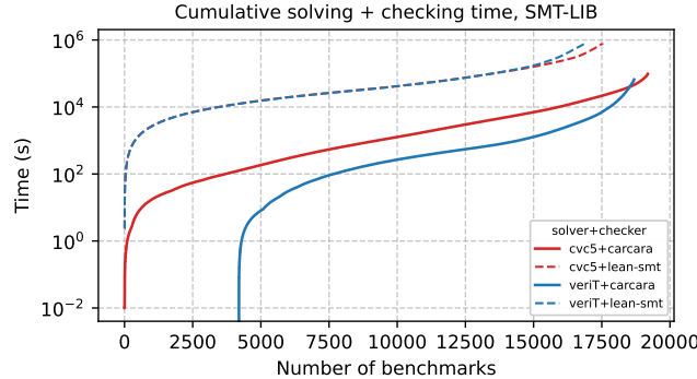
Fig. 3. Cumulative solving and checking time against the number of SMT-LIB benchmarks whose proof the configuration validated. CARCARA validates 19 190 CVC5 proofs in 26.9 CPU hours and 18 685 VERiT proofs in 18.3; the checker validates 17 540 and 16 921 in 220 and 228.
