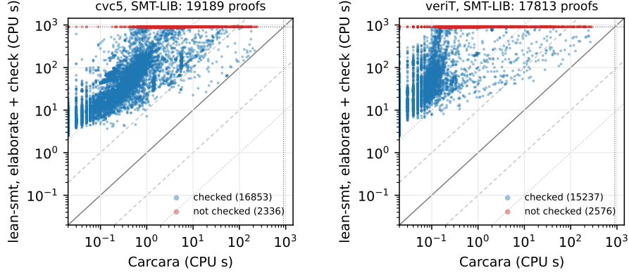
Fig. 2. CARCARA’s check of the solver’s proof against the elaboration plus LEAN-SMT’s check, on the SMT-LIB proofs CARCARA accepts, CPU seconds. Red points are proofs the checker did not finish within its limit; the grey lines are equality and factors of ten and a hundred.
