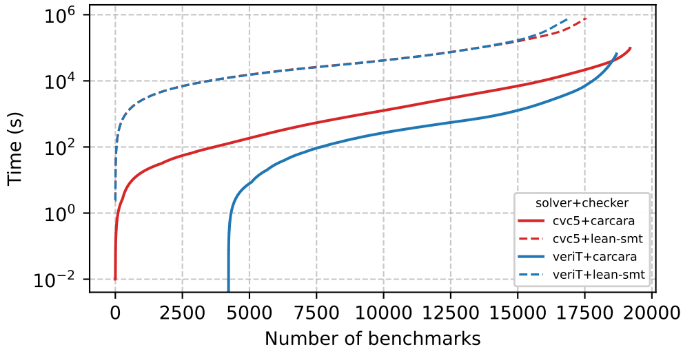
Cumulative solving + checking time, SMT-LIB
