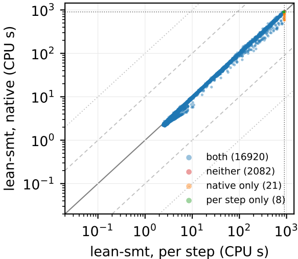
veriT, SMT-LIB: 19031 proofs
