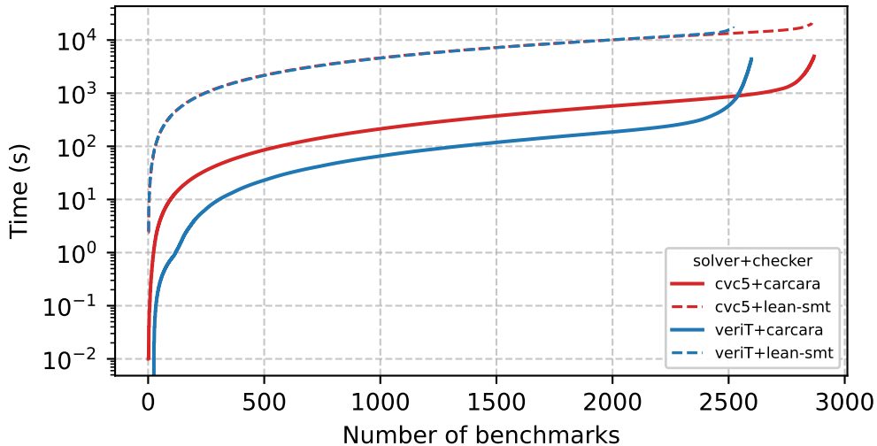
Cumulative solving + checking time, Sledgehammer
