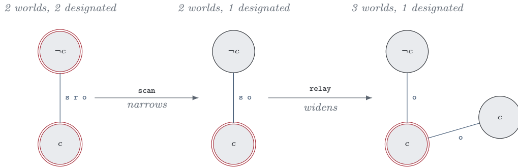
Figure 2: The model at each step. A double ring marks a designated world; an edge is labelled with the agents that cannot distinguish its endpoints. The counts are those the run reported.
