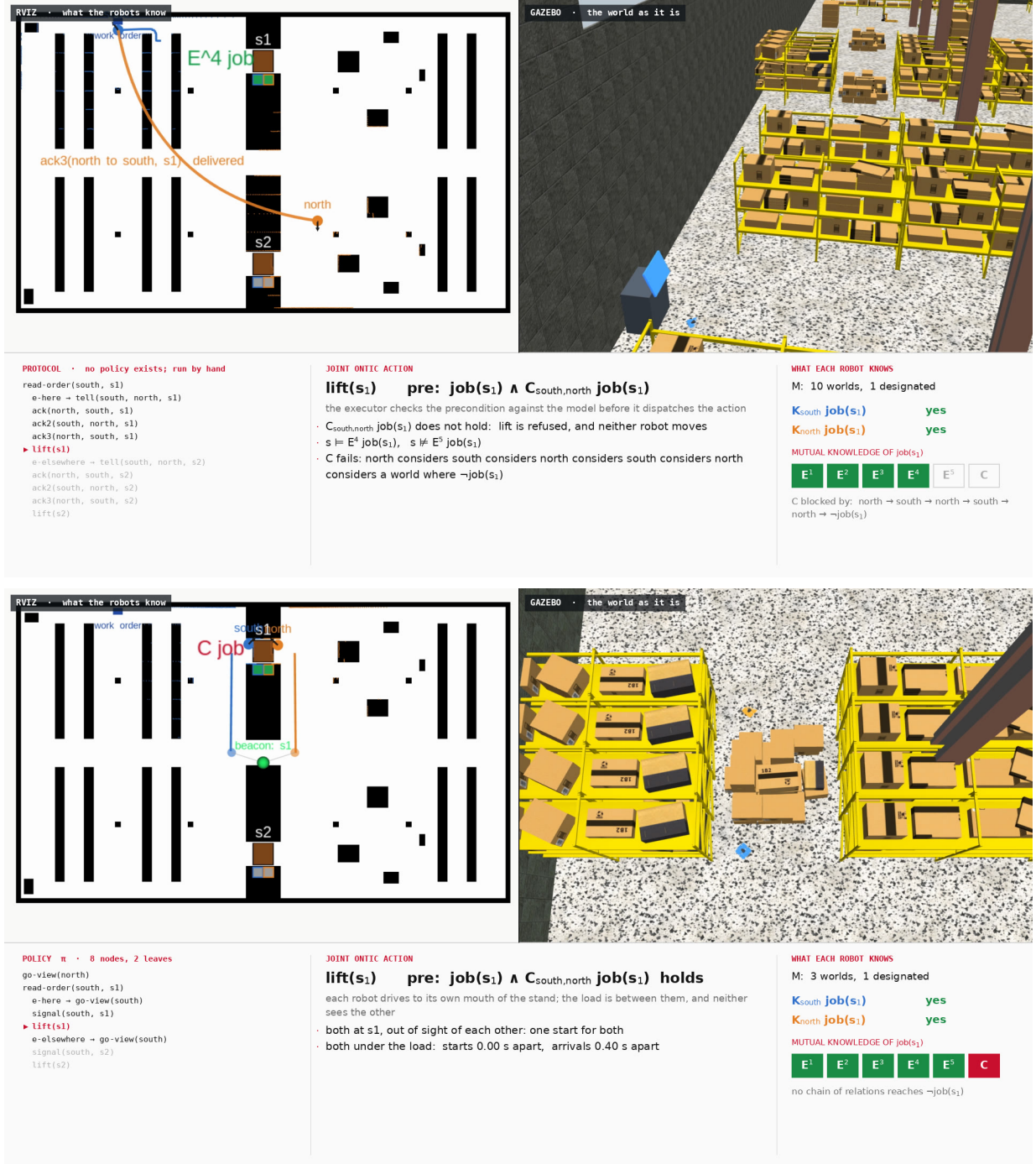
Figure 6: Two frames of the film. Above, the radio floor after the fourth message: E^4 , and the lift refused. Below, the beacon floor during the lift, seen from above the bay: C , both robots under the load.
