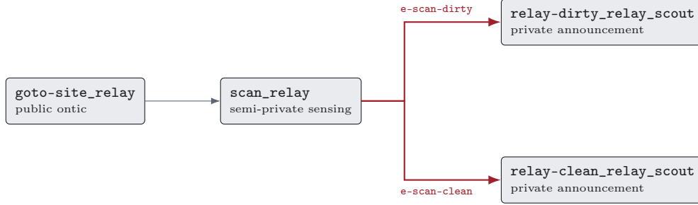
Figure 1: The four-node policy. The branch is on an observation rather than on a state variable, and both arms announce privately.
