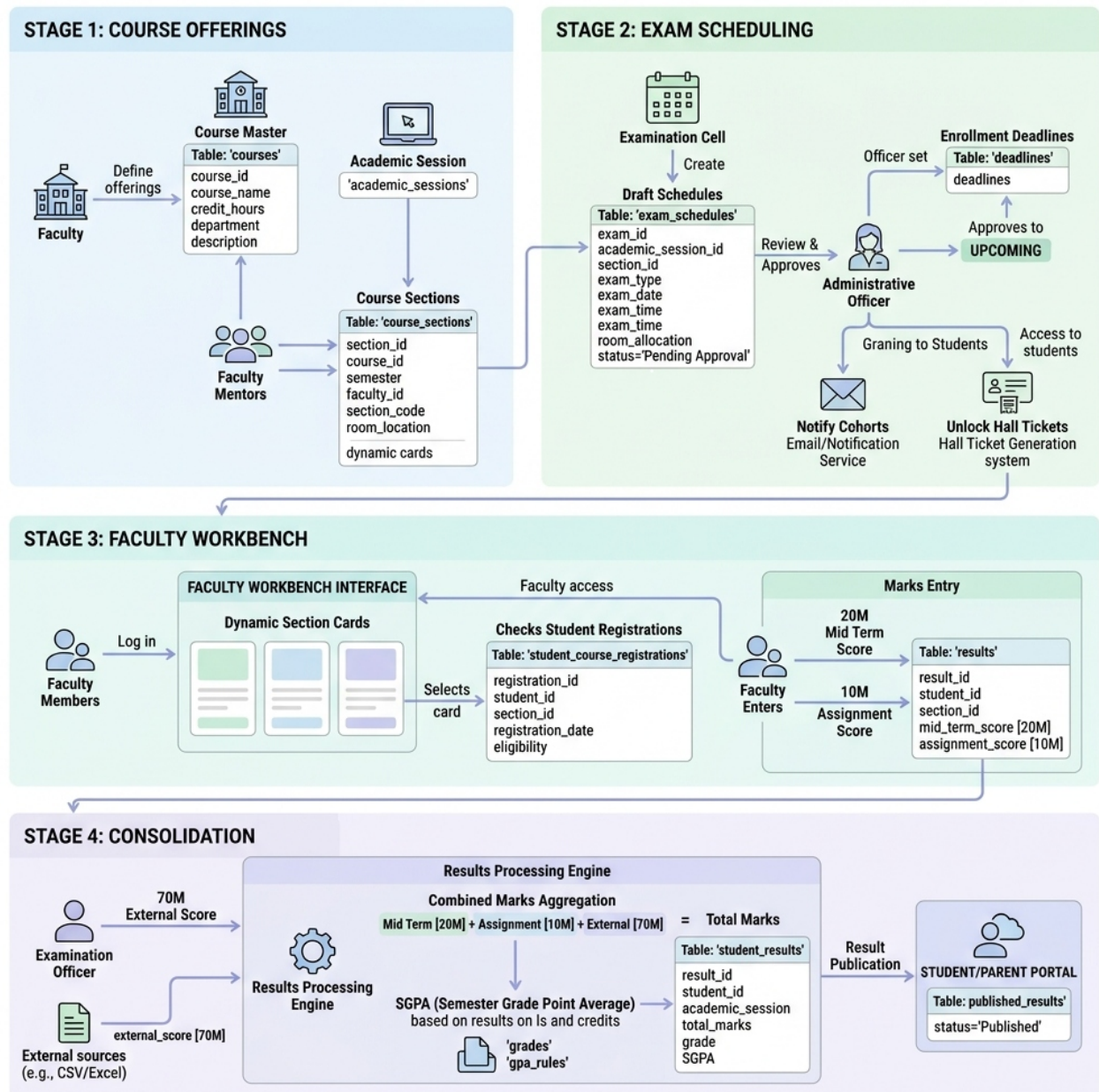
Figure 3.1: Examination Scheduling, Marks Entry and Aggregation Stages
