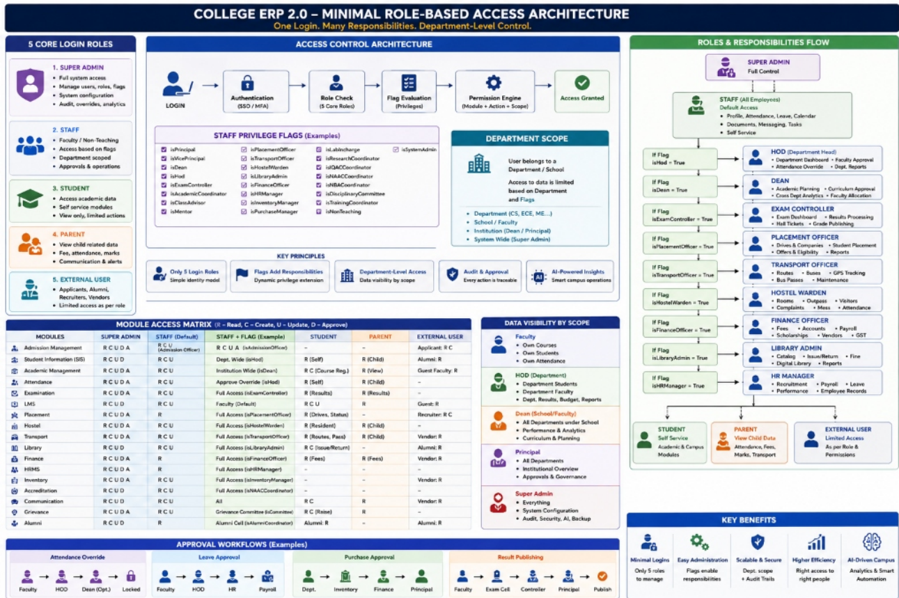
Figure 5.1: College ERP 2.0 Access Control Architecture & Responsibility Matrix
