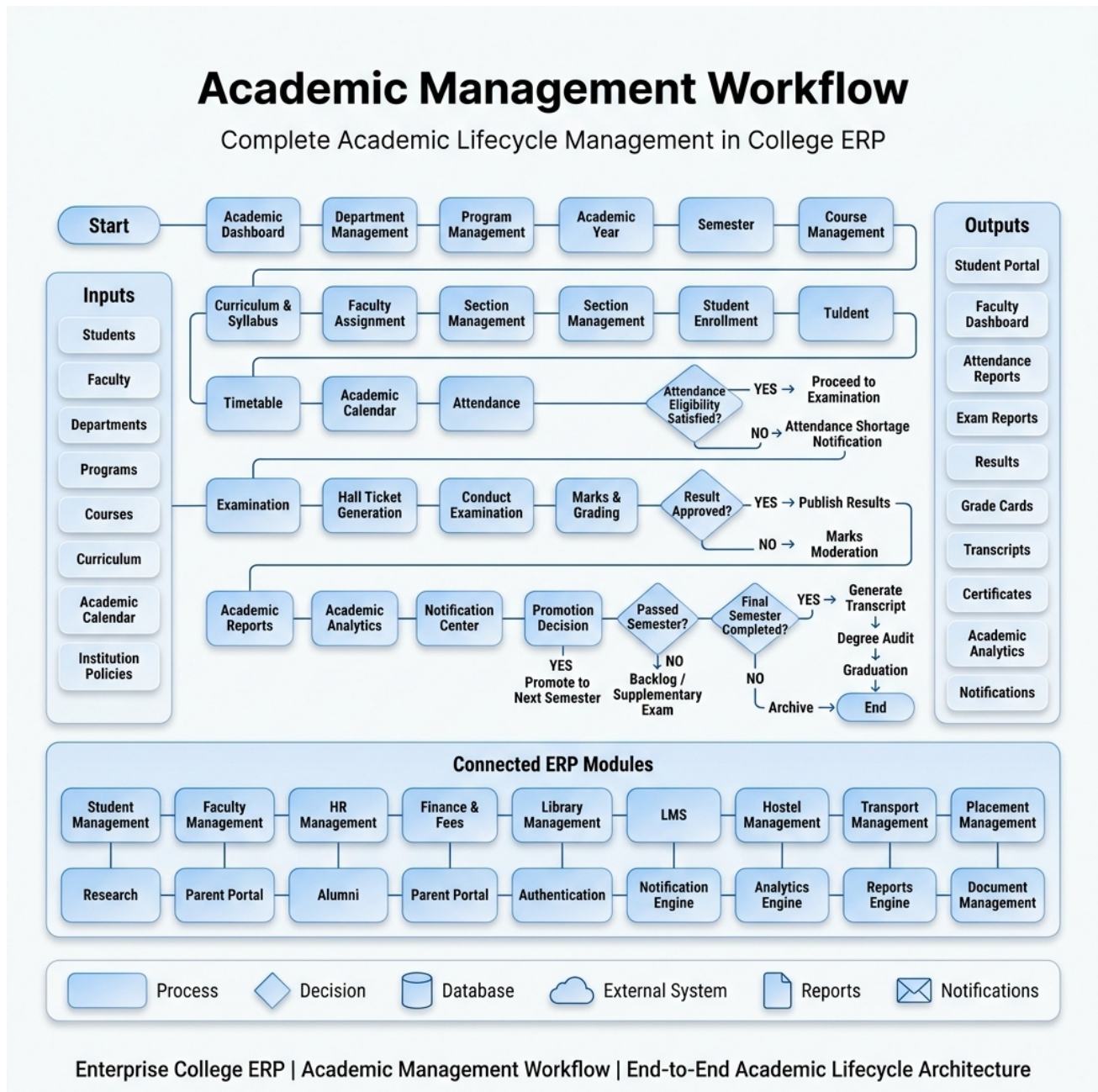
Figure 1.1: Academic Management Lifecycle & Module Connections
