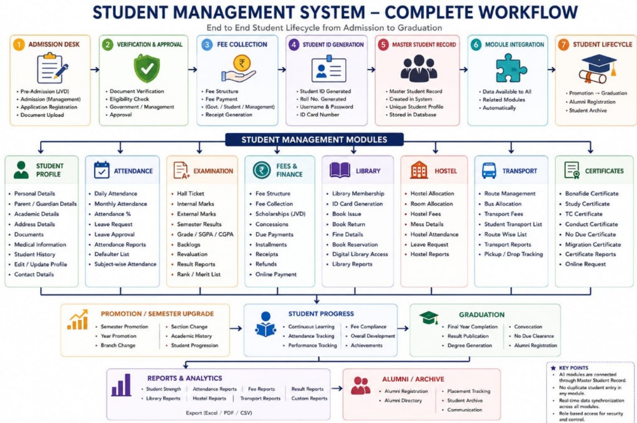
Figure 4.1: End-to-End Student Lifecycle Workflow and Core Module Integrations
