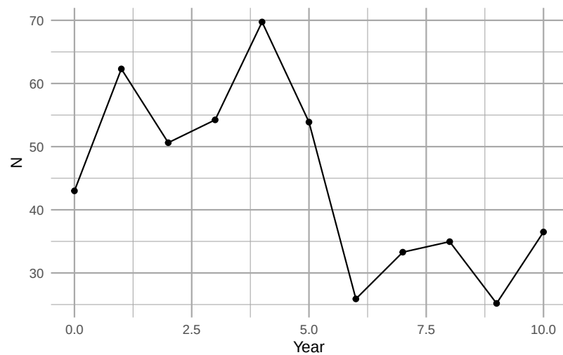
Figure 4.10: A single simulated population projection.
