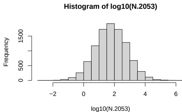
Figure 4.13: Distribution of the 10000 final base-10 log population sizes. Note the approximately Normal distribution.
