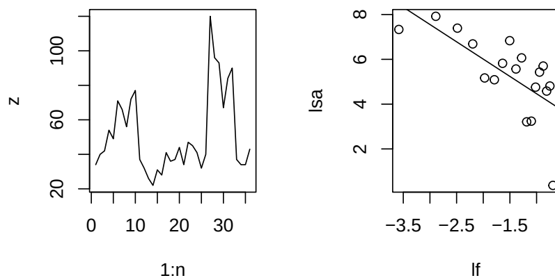
Figure 4.20: Sparrow population dynamics seems to show reddened fluctuations. On the left, sparrow counts over time, and on the right, the log-log plot of the power spectrum (power vs. frequency). The frequentist confidence interval on the slope of the fitted line suggests that we shouldn't rule out the possibility of a reddened series.
