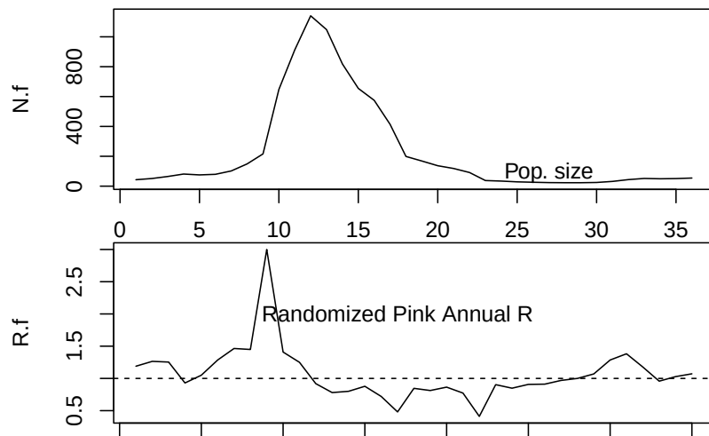
Figure 4.22: Example of a simulated sparrow projection using reddened annual growth rates.
