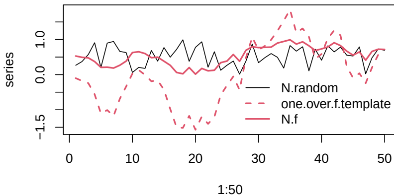
Figure 4.19: Example of spectral mimicry, showing the original random data points (solid black line), the template ('one.over.f.template', red dashed line), and the rearranged, reddened data points (solid red line).
