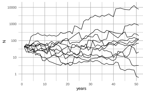
Figure 4.12: Using ggplot() to plot one variable against vs. a single variable, organized by a grouping variable. Our simulated populations sometimes increase and sometimes decrease.
