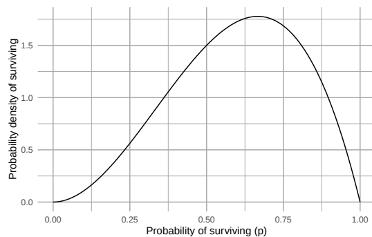
Figure 4.14: Our prior belief on the probability that the Song Sparrow population in Darrrtown will replace itself over our time interval. We call this the prior probability distribution .
