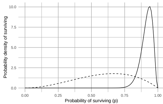
Figure 4.15: Our updated beliefs (solid line) about the probability that the Song Sparrows will replace themselves over our time interval. The solid line is the posterior distribution. The dashed line was our prior beliefs or prior distribution.
