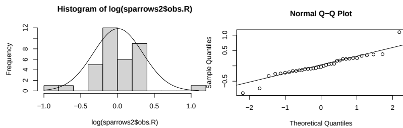
Figure 4.16: The logarithms of the observed R arrayed in a histogram (left) and a quantile-quantile plot comparing our log-growth rates to the normal distribution (right). Our data seem somewhat approximated by a Normal distribution whose mean and standard deviation are derived from the log-transformed data. The probability distribution has been rescaled to be visible on this graph. However, the q-q plot shows that the sample (y-axis) includes values that are smaller and larger than predicted by the normal distribution.
