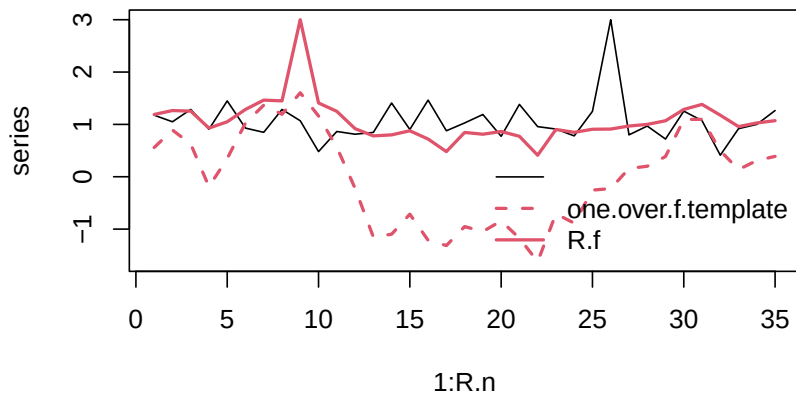
Figure 4.21: Original and rearranged annual growth rates.
