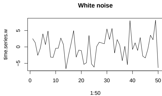
Figure 4.18: Examples of reddened (left) and white (right) time series.
