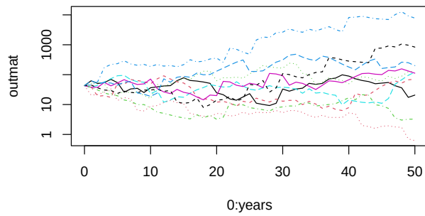
Figure 4.11: Using matplot() to plot a matrix vs. a single variable. Our simulated populations sometimes increase and sometimes decrease.
