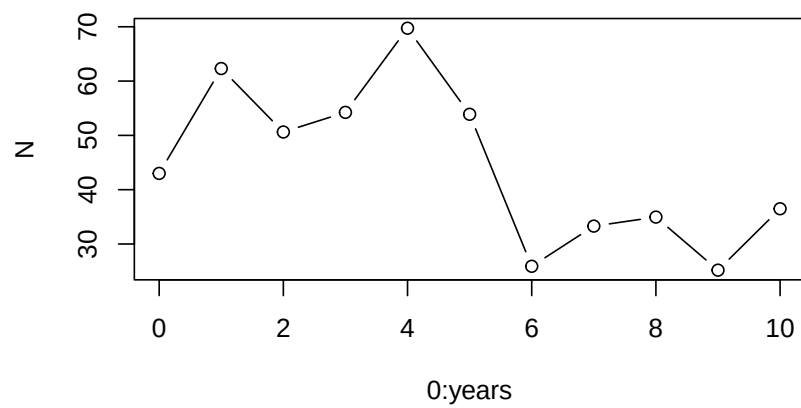
Figure 4.9: A single simulated population projection.
