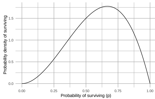
Figure 4.12: Our prior belief on the probability that the Song Sparrow population in Darrrtown will replace itself over our time interval. We call this the prior probability distribution .
