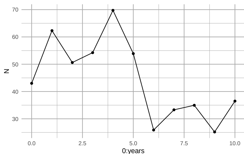
Figure 4.8: A single simulated population projection.
