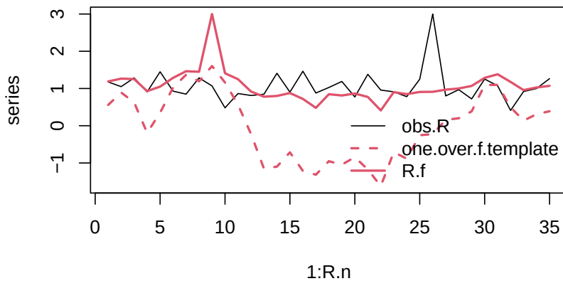
Figure 4.19: Original and rearranged annual growth rates.
