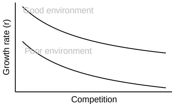
Superadditive
