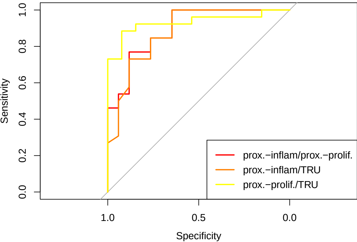
Random Forest Classifier ROC-Curve
