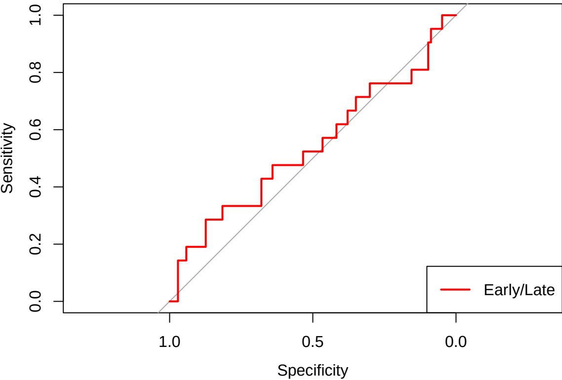
Binomial Logistical Regression ROC-Curve
