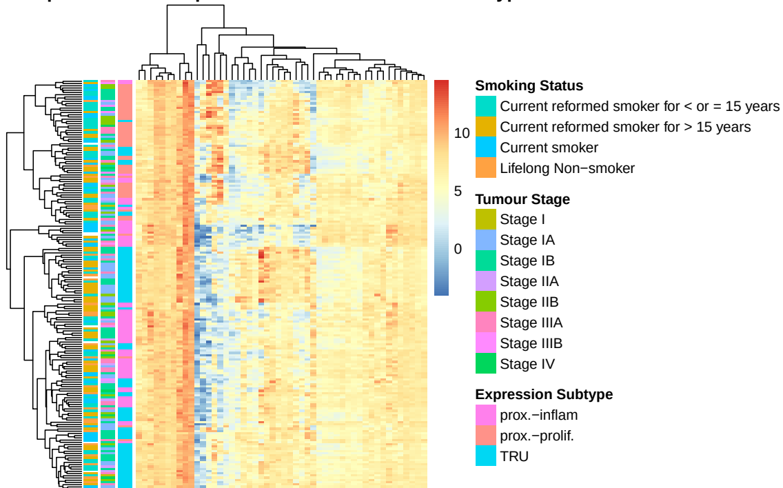
Expression heatmap of the TOP 50 DEGs across subtypes
