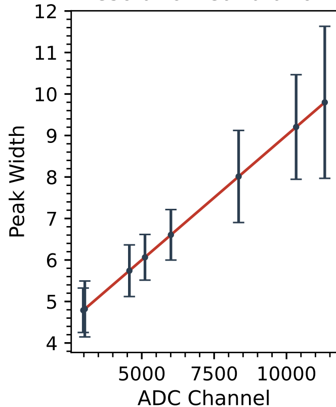
Resolution Calibration
