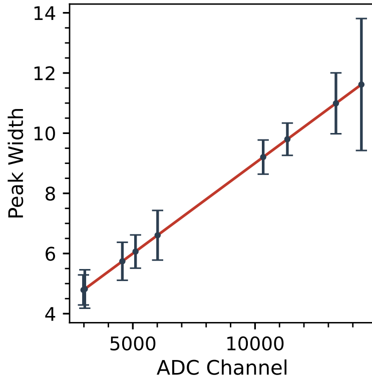
Resolution Calibration
