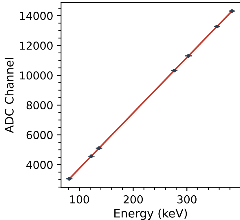
Energy Calibration
