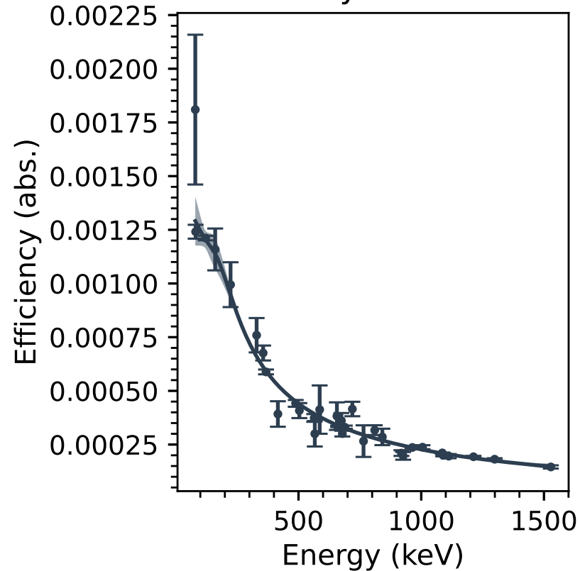
Efficiency Calibration
