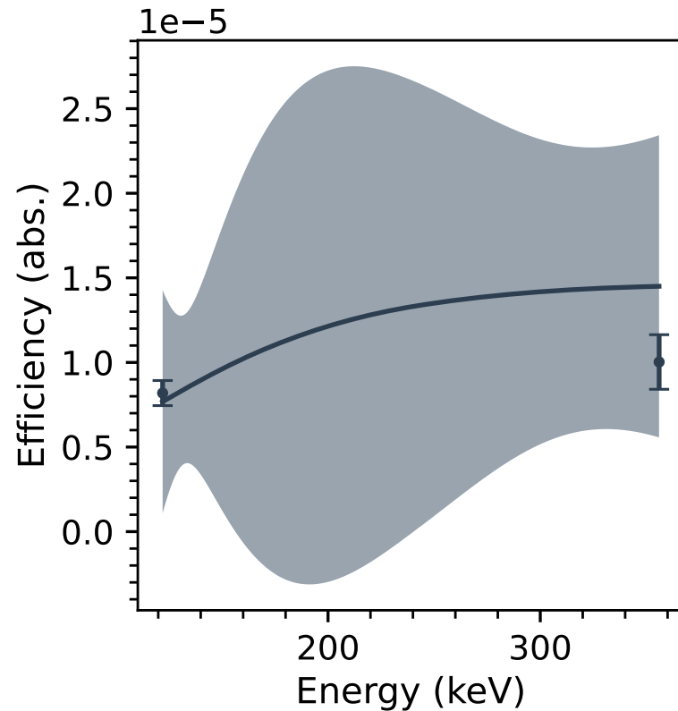
Efficiency Calibration
