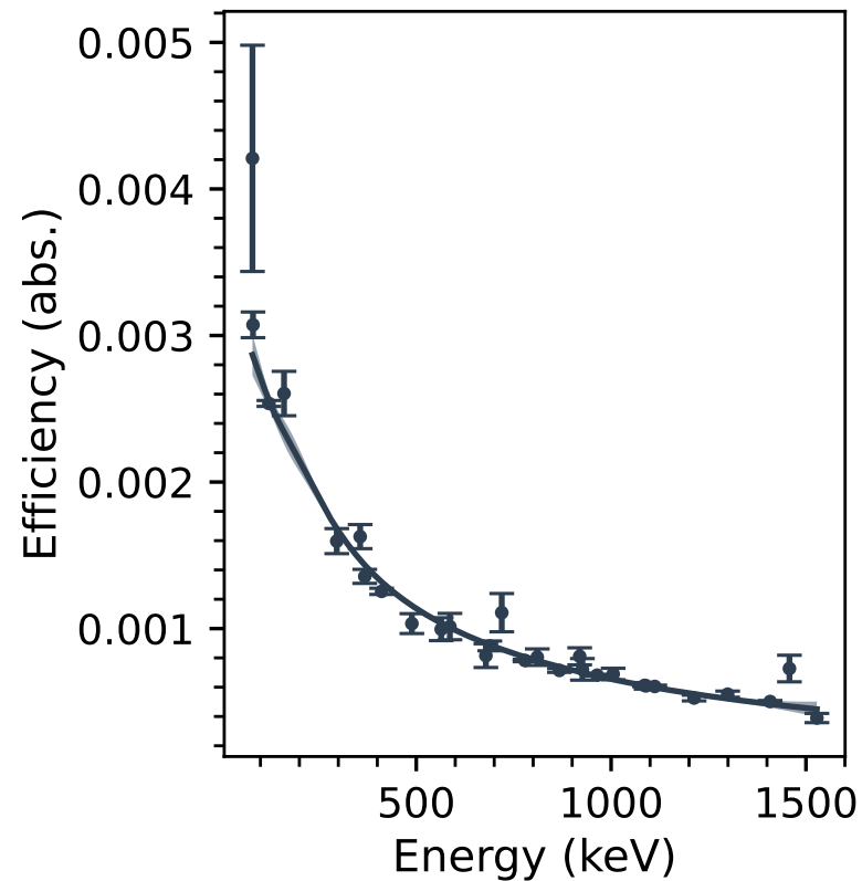
Efficiency Calibration
