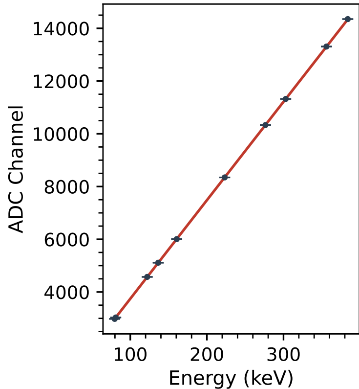
Energy Calibration
