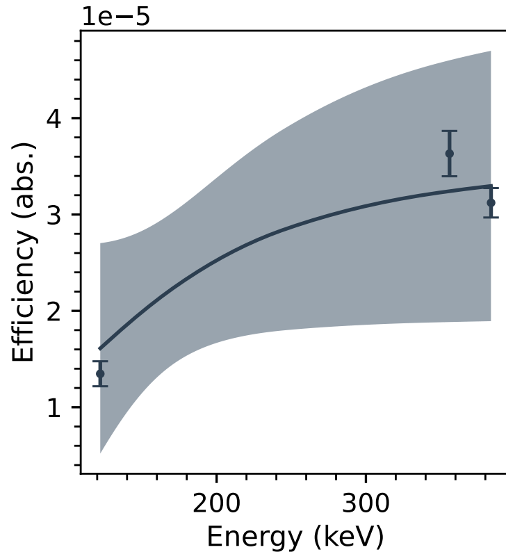
Efficiency Calibration
