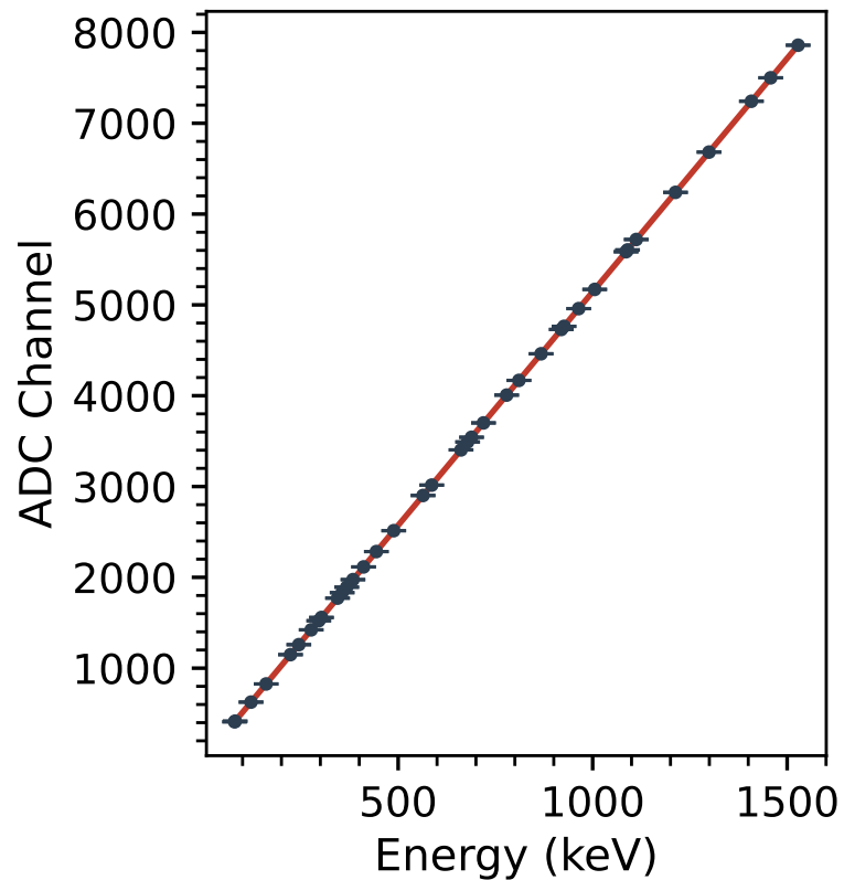
Energy Calibration
