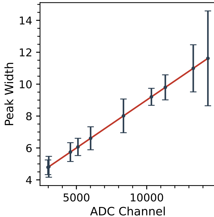
Resolution Calibration
