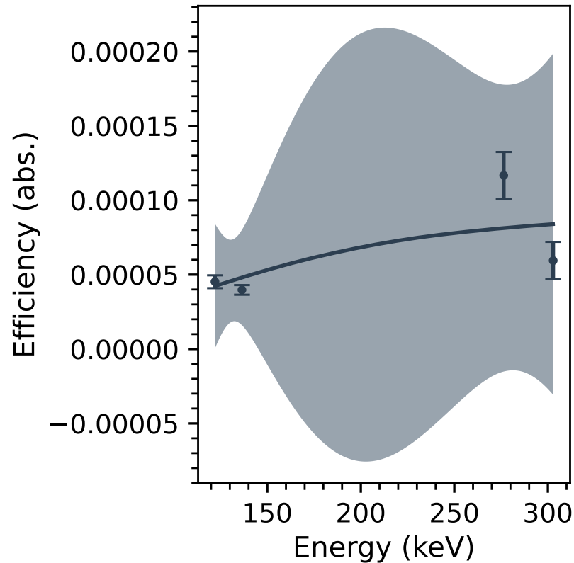
Efficiency Calibration
