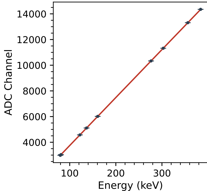
Energy Calibration
