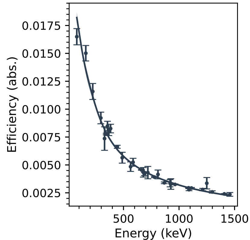
Efficiency Calibration
