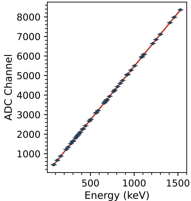
Energy Calibration
