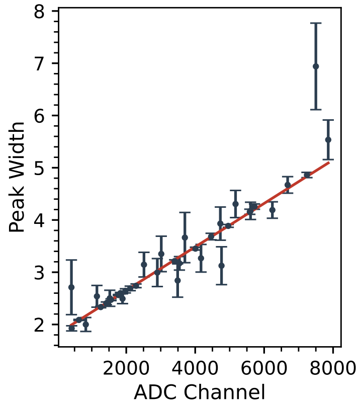
Resolution Calibration
