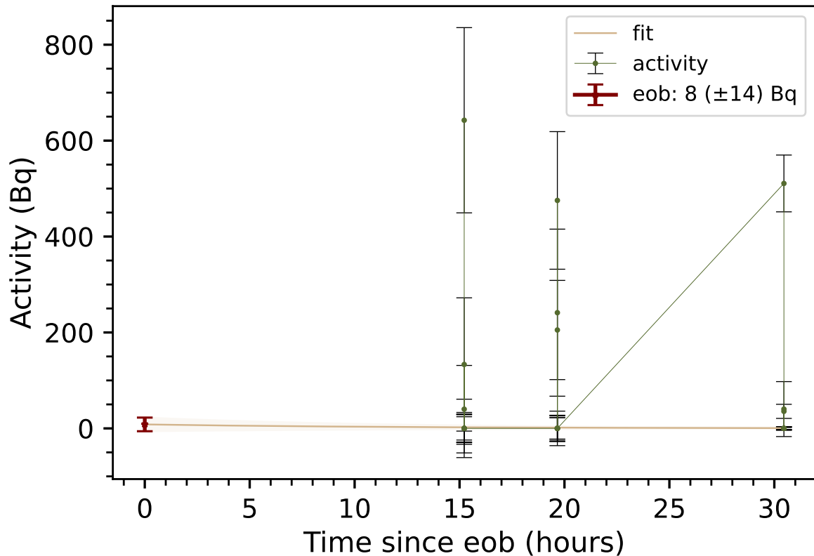
Ta 176TA Ta06 - cumulative
