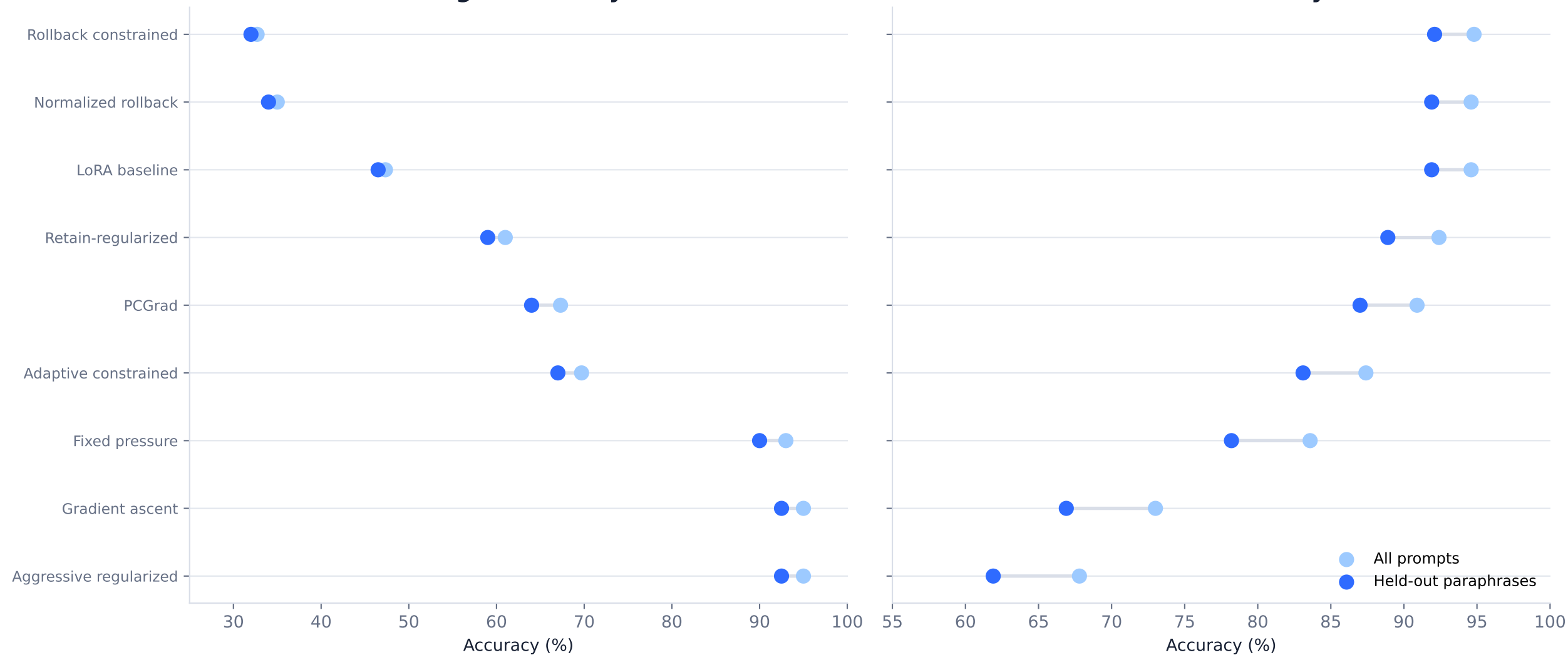
Forget accuracy
