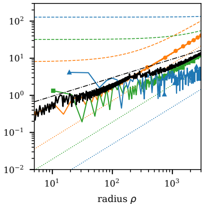
(b) chains of Theorem 2
