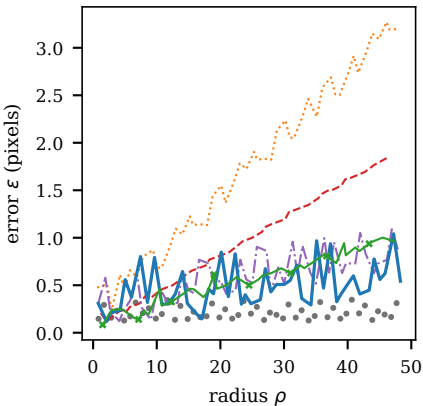
(a) families, \rho \leq 48
