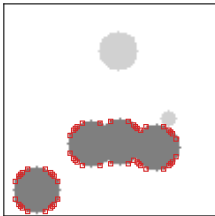
(a) disk particles X
