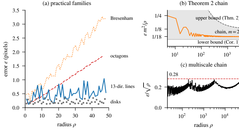
Fig. 2. Roundness error \varepsilon of single-element chains. (a) Practical families (all in Table 2); the disks used by the sup-closure for reference. (b) The chain of Theorem 2 with m = 2 , normalised by \rho/m^2 , settles at about 1/18 between the bounds of Theorem 2 and Corollary 1. (c) The multiscale chain, normalised by \sqrt{\rho} , stays below 0.28
