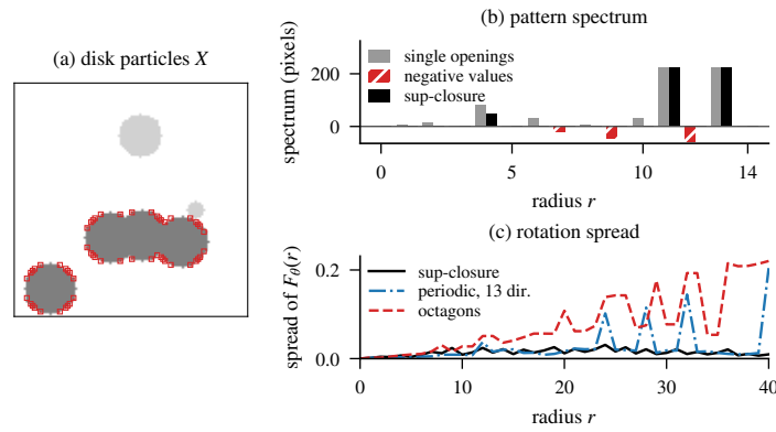
Fig. 3. (a) Disk particles X (light grey), X \circ D_{12} (dark grey), and pixels of X \circ D_{13} not in X \circ D_{12} (red). (b) Pattern spectrum of X : single disk openings give negative values, the sup-closure does not (two bars clipped). (c) Rotation spread \max_\theta F_\theta - \min_\theta F_\theta on the squares scene
