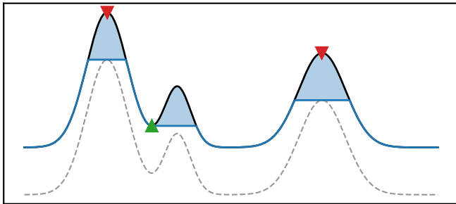
(a) provenance of the h -dome, 1-D
