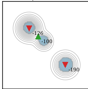
(b) \nabla_u \sum_p D_h(u)(p) , 2-D
