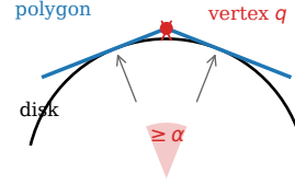
(c) gap \Rightarrow not round
