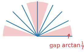
(b) directions, \|v\| \leq 3
