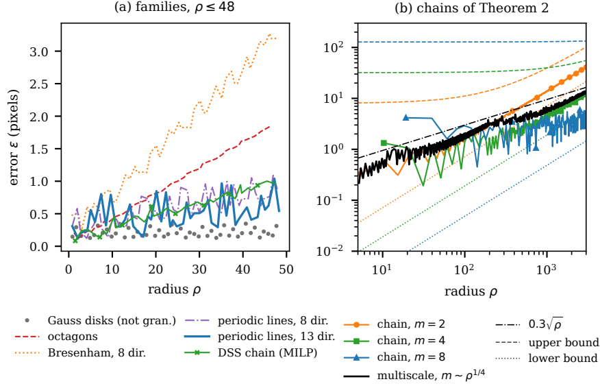
Fig. 2. (a) Error of practical families for \rho \leq 48 ; mean-radius steps are below 2.2. (b) Chains of Theorem 2 for m = 2, 4, 8 , with the upper bound of Theorem 2 (dashed) and the lower bound of Corollary 1 (dotted), and the multiscale chain against 0.3\sqrt{\rho} .
