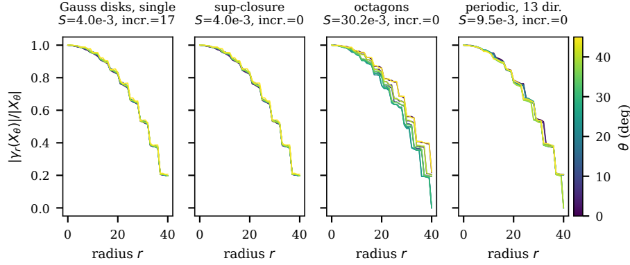
Fig. 3. Size distributions of the rotated synthetic scene, one curve per angle. Single openings by Gauss disks are nearly isotropic but non-monotone. Their sup-closure removes the increases and keeps the isotropy. Octagons are monotone but orientation dependent, and the 13-direction periodic chain reduces this dependence by a factor of three.
