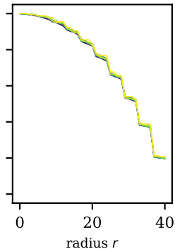
sup-closure of Gauss disks S=4.0\text{e-}3 , increases=0
