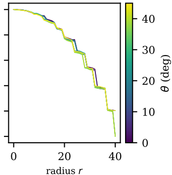
periodic lines, 13 dir. S=9.5\text{e-}3 , increases=0
