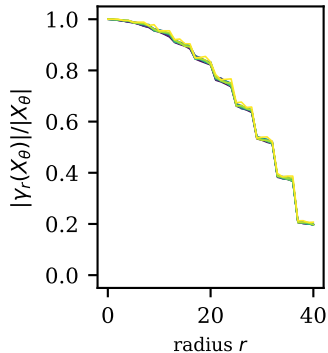
Gauss disks (single) S=4.0\text{e-}3 , increases=17
