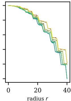
octagons S=30.2\text{e-}3 , increases=0
