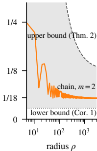
(b) Theorem 2 chain
