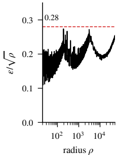
(c) multiscale chain
