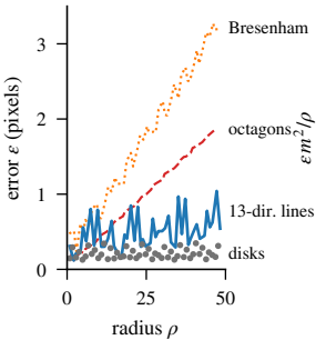
(a) practical families
