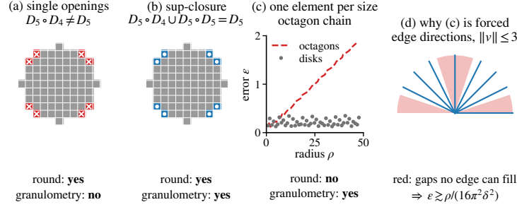
Fig. 1. Overview. (a) Common practice: the red pixels of D_5 lie in no translate of D_4 inside D_5 , so absorption fails. (b) The sup-closure also opens by larger disks and recovers them (Proposition 1). (c) One element per size gives a granulometry whose error grows with the radius. (d) This is unavoidable (Theorem 1): short lattice vectors leave gaps of \arctan(1/\ell) next to the axes
