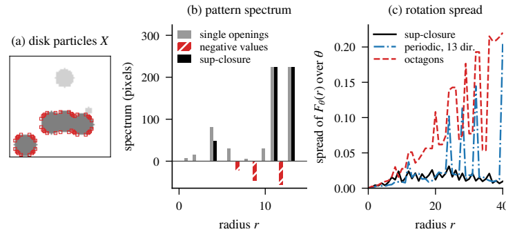
Fig. 3. (a) Disk particles X (light grey), X \circ D_{12} (dark grey), and pixels of X \circ D_{13} not in X \circ D_{12} (red). (b) Pattern spectrum of X : single disk openings give negative values, the sup-closure does not (two bars clipped). (c) Rotation spread \max_\theta F_\theta - \min_\theta F_\theta on the squares scene
