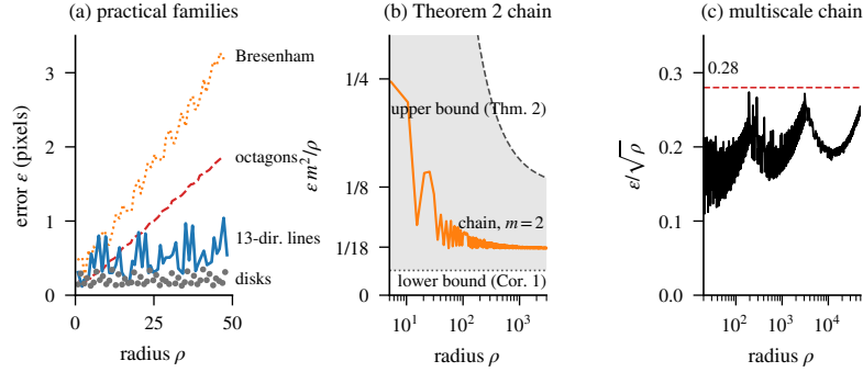
Fig. 2. Roundness error \varepsilon of single-element chains. (a) Practical families (all in Table 2); the disks used by the sup-closure for reference. (b) The chain of Theorem 2 with m = 2 , normalised by \rho/m^2 , settles at about 1/18 between the bounds of Theorem 2 and Corollary 1. (c) The multiscale chain, normalised by \sqrt{\rho} , stays below 0.28
