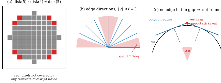
Fig. 1. (a) The digital disk of radius 5 is not open with respect to that of radius 4: the red pixels lie in no translate of the smaller disk that fits inside. (b) Idea of Theorem 1: lattice vectors of norm at most \ell (here 3) leave gaps of \arctan(1/\ell) next to the axes. (c) A polygon whose edges come from such vectors has no edge with a direction in the gap. Over the corresponding range of normals a single vertex carries the support and sticks out of the circle (schematic, gap exaggerated).
