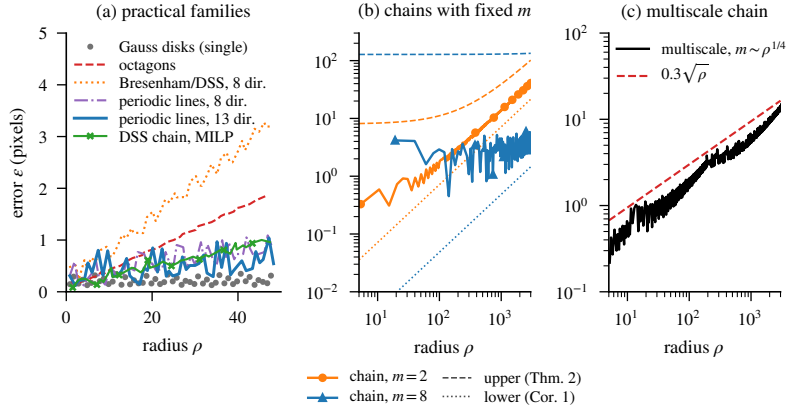
Fig. 2. Roundness error \varepsilon of single-element chains. (a) Practical families (mean-radius steps below 2.2); Gauss disks for reference. (b) Chains of Theorem 2 for m = 2, 8 (solid) lie between the upper bound of Theorem 2 (dashed) and the lower bound of Corollary 1 (dotted), both growing linearly. (c) The multiscale chain grows only like \sqrt{\rho}
