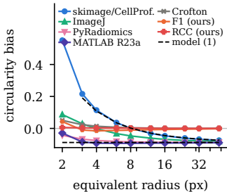
(b) 2D, synthetic
