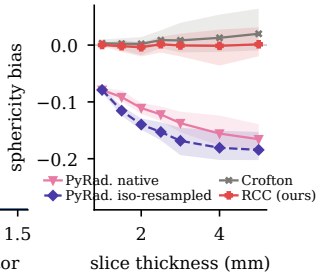
(e) 3D, synthetic, R \geq 5 mm
