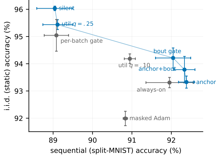
Figure 6: The operating frontier under the stateless optimiser: split-MNIST sequential accuracy against i.i.d. static accuracy (six seeds on the bout-gate and always-on points, three elsewhere). Blue: non-dominated configurations; grey: dominated ones. No single configuration wins both axes; the bout-committed gate is the sequential-side default, silent isolation the static-side one.
