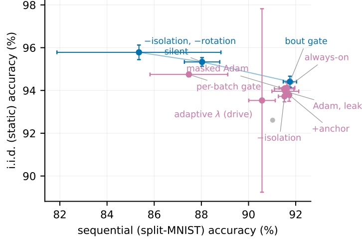
Figure 5: The operating frontier at the record fraction under heavy-ball SGD: split-MNIST sequential accuracy against i.i.d. static accuracy (headline points six seeds). Blue: non-dominated by seed means (the bout-committed gate, the silent mask, unmasked rotation-free replay); purple: dominated; held-out split. The top cluster (always-on rotation, bout gate, anchor, masked Adam) lies within seed noise of one another; the frontier trades sequential for static accuracy through the silent and unmasked variants, and the adaptive- \lambda point (Section 7) is dominated on this split.
