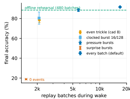
Figure 3: Replay timing at sparse budgets: accuracy against the number of waking replay events; trickles and clocked bursts fail alike, pressure-triggered bursts (star) keep most of the accuracy at a third of the events, surprise triggering fires no events in this regime.
