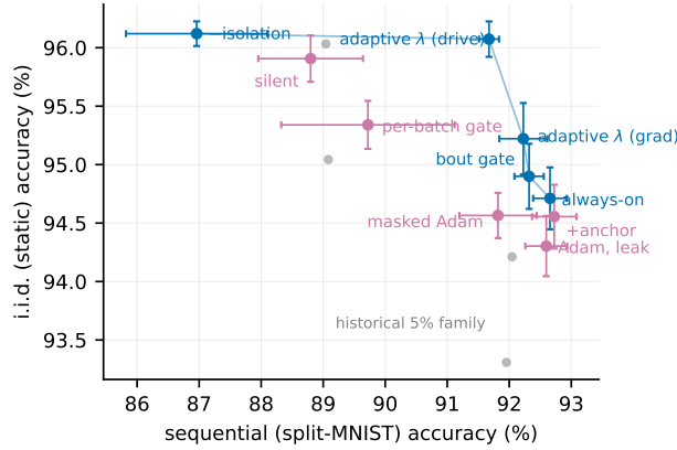
Figure 4: Operating frontier at the 10% activity fraction under heavy-ball SGD: split-MNIST sequential accuracy against i.i.d. static accuracy. Blue: non-dominated configurations; purple: dominated; grey: the 5% family of earlier phases. No single configuration wins both axes; always-on rotation is the sequential default and the adaptive decay extends the static side.
