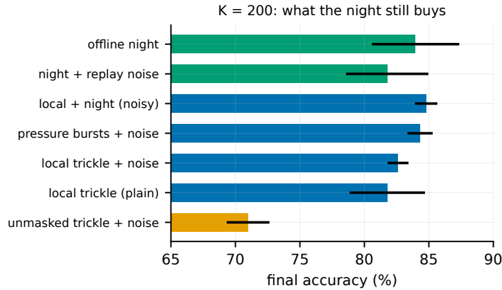
Figure 9: K = 200 mechanism triangulation. Isolated rotating replay beats the unmasked trickle, diversity helps only during wake, and the irreducible advantage of the night at tiny buffers is its interference-free window.
