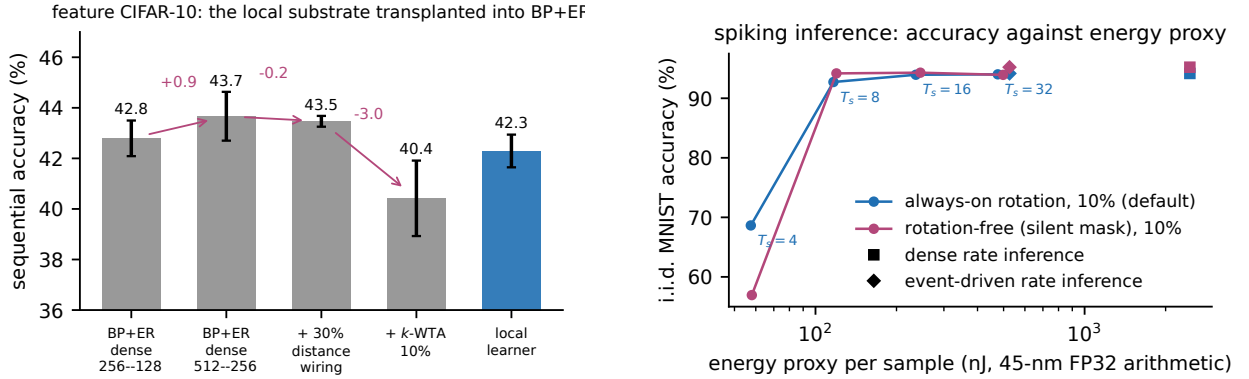
Figure 7: Left: the substrate decomposition on feature CIFAR-10, transplanting the local network’s ingredients into BP+ER one at a time (each cell at its better of two learning rates; three seeds). Right: spiking inference, i.i.d. MNIST accuracy against the idealised 45-nm FP32 arithmetic-energy proxy for T_s \in \{4, 8, 16, 32\} , with the dense (square) and event-driven (diamond) rate references; held-out split; the default is monotone in T_s , the rotation-free control dips 0.4 at T_s=32 .
