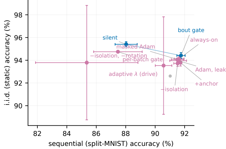
Figure 6: The operating frontier at the 10% fraction under heavy-ball SGD: split-MNIST sequential accuracy against i.i.d. static accuracy (headline points six seeds). Blue: non-dominated by seed means (the bout-committed gate and the silent mask); purple: dominated; held-out split. The top cluster (always-on rotation, bout gate, anchor, masked Adam) lies within seed noise of one another; the frontier trades sequential for static accuracy through the silent mask, the unmasked rotation-free control is dominated by it once its collapsed seed is counted, and the adaptive- \lambda point (Section 7) is dominated on this split.
