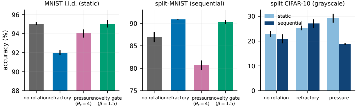
Figure 8: Rotation: price, trade-off, and gate. Left: on i.i.d. MNIST the novelty gate restores no-rotation accuracy. Middle: on split-MNIST rotation is required and the gate keeps it. Right: on split CIFAR-10 (grayscale) rotation is a gain on both axes.
