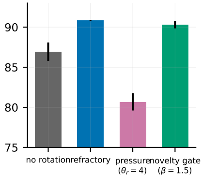
split-MNIST (sequential)
