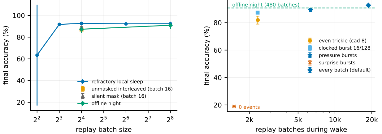
Figure 4: Left (isolation): final split-MNIST accuracy vs. replay batch size (record substrate, heavy-ball SGD). Masked refractory replay is insensitive down to 8 samples; unmasked, silent-masked and offline-night replay all degrade. Right (timing): accuracy vs. number of waking replay batches. Even trickles fail; clocked bursts recover most of the gap; pressure-triggered bursts (star) dominate at sparse budgets; surprise triggering never fires at all.
