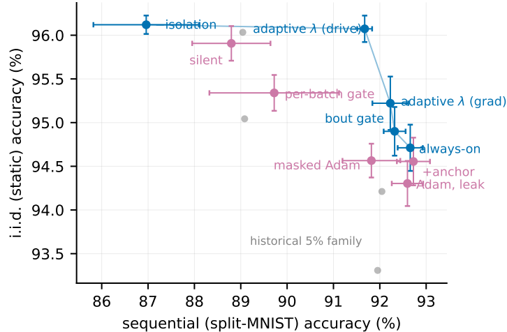
Figure 5: The operating frontier at the record fraction under heavy-ball SGD: split-MNIST sequential accuracy against i.i.d. static accuracy (headline points six seeds). Blue: non-dominated configurations; purple: dominated ones; small grey dots: the 5% family of the earlier phases, entirely inside the new frontier. The two adaptive- \lambda points (Section 7) extend the static side of the frontier and retire the silent mask and the per-batch gate. No single configuration wins both axes; always-on rotation is the sequential default.
