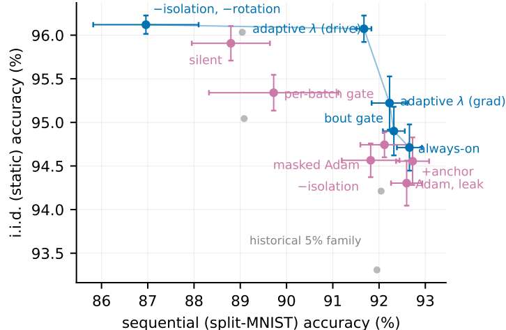
Figure 5: The operating frontier at the record fraction under heavy-ball SGD: split-MNIST sequential accuracy against i.i.d. static accuracy (headline points six seeds). Blue: non-dominated configurations; purple: dominated ones; small grey dots: the 5% family of the earlier phases, entirely inside the new frontier. The two adaptive- \lambda points (Section 7) extend the static side of the frontier and retire the silent mask and the per-batch gate. No single configuration wins both axes; always-on rotation is the sequential default.
