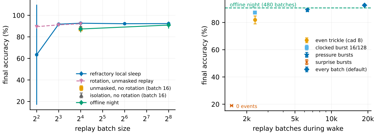
Figure 4: Left (isolation): final split-MNIST accuracy vs. replay batch size (record substrate, heavy-ball SGD); the number of updates is fixed within each series (one per waking batch; 20 per epoch for the night, whose samples therefore fall with its batch). The full system is insensitive down to 8 samples; rotation with unmasked replay (dashed) trails it by 0.6 at 8–16 and holds at 4, where the masked system turns bimodal; without rotation, unmasked and isolated replay and the offline night all degrade. Right (timing): accuracy vs. number of waking replay batches. Even trickles fail; clocked bursts recover most of the gap; pressure-triggered bursts (star) dominate at sparse budgets; surprise triggering fires no events in this regime.
