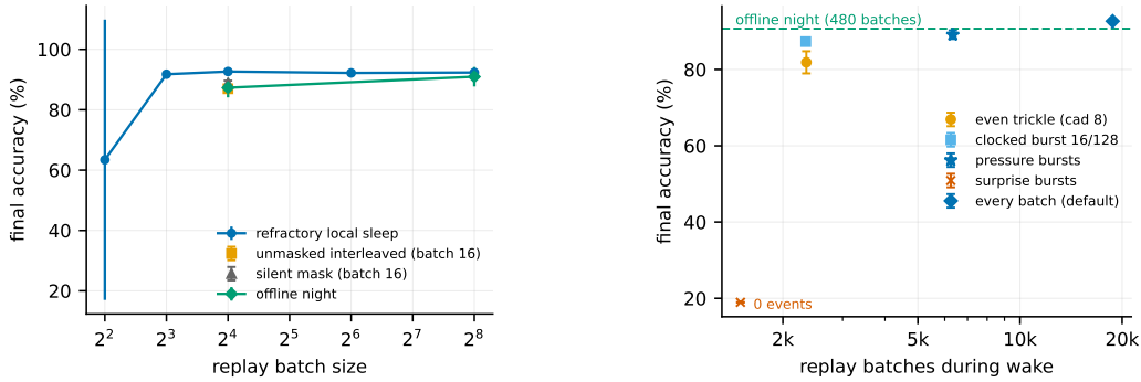
Figure 2: Left (isolation): split-MNIST accuracy against replay batch size: masked refractory replay is insensitive down to 8 samples; unmasked, silent-masked and offline-night replay degrade. Right (timing): accuracy against the number of waking replay events: trickles fail, clocked bursts recover most of the gap, pressure-triggered bursts (star) dominate at sparse budgets, surprise triggering fires no events in this regime.
