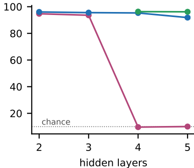
i.i.d. (static)
