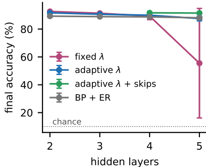
sequential (split-MNIST)
