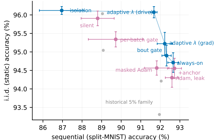
Figure 4: The operating frontier at the record fraction under the stateless optimiser: split-MNIST sequential accuracy against i.i.d. static accuracy (headline points six seeds). Blue: non-dominated configurations; purple: dominated ones; small grey dots: the historical 5% family the project inherited, entirely inside the new frontier. The two adaptive- \lambda points (Section 7) extend the static side of the frontier and retire the silent mask and the per-batch gate. No single configuration wins both axes; always-on rotation is the sequential default.
