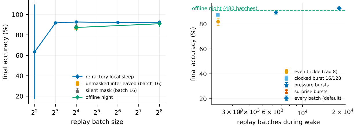
Figure 3: Left (isolation): final split-MNIST accuracy vs. replay batch size (record substrate, stateless SGD). Masked refractory replay is insensitive down to 8 samples; unmasked, silent-masked and offline-night replay all degrade. Right (timing): accuracy vs. number of waking replay batches. Even trickles fail; clocked bursts recover most of the gap; pressure-triggered bursts (star) dominate at sparse budgets; surprise triggering never fires at all.
