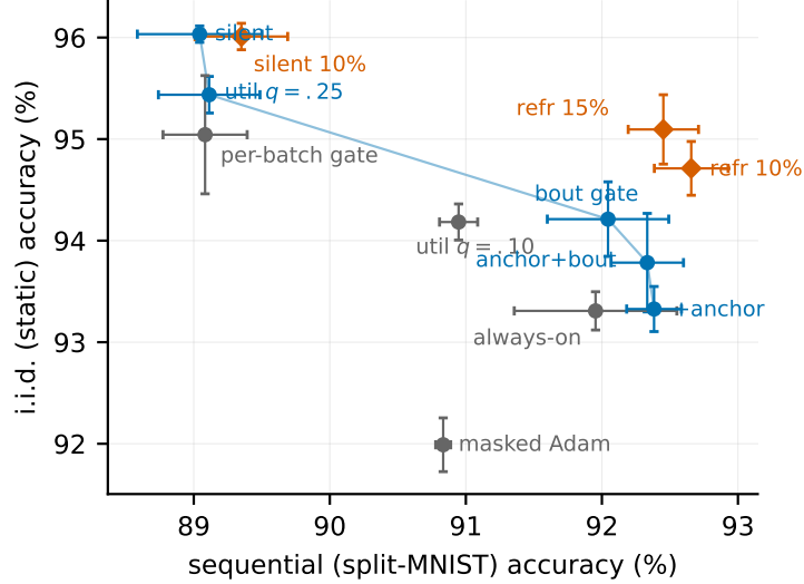
Figure 6: The operating frontier under the stateless optimiser: split-MNIST sequential accuracy against i.i.d. static accuracy (six seeds on the bout-gate, always-on and dial points, three elsewhere). Blue: non-dominated configurations at the historical 5% activity fraction; grey: dominated ones; orange diamonds: the same machinery with the k -WTA fraction relaxed to 10–15% (Section 6.4), which shifts the whole frontier outward. Within a fraction, no single configuration wins both axes.
