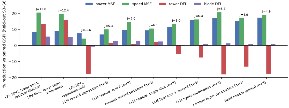
Figure 2: What each controller’s J is made of (held-out S3–S6, arm means). Every fixed-reward and hyper-parameter arm buys regulation with tower fatigue; the reward-expression agent and the correctly scaled MPC are the rows with every term positive.
