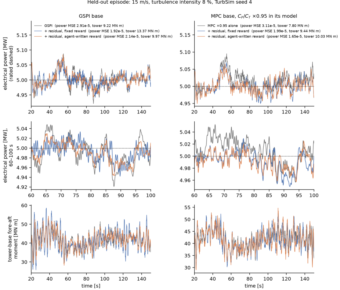
Figure 3: One held-out above-rated episode, both bases: how close each controller holds power to rated, and what it costs the tower. Rows: electrical power over the scored window (rated dashed); the same, 60–100 s; tower-base fore-aft moment. Columns: the GSPI base with GSPI, the fixed-reward residual and the agent-reward residual (one seed each, the seed nearest its arm’s mean); the MPC with the 5 % model error alone and with the two residuals. The legend gives the episode’s power MSE on above-rated steps and its tower-base fatigue; above rated the generator torque is constant, so the generator-speed trace is the power trace scaled and its MSE is the same number. The episode is the 15 m/s realisation on which the two GSPI-base arms’ tower-fatigue difference is closest to its mean over the four held-out realisations.
