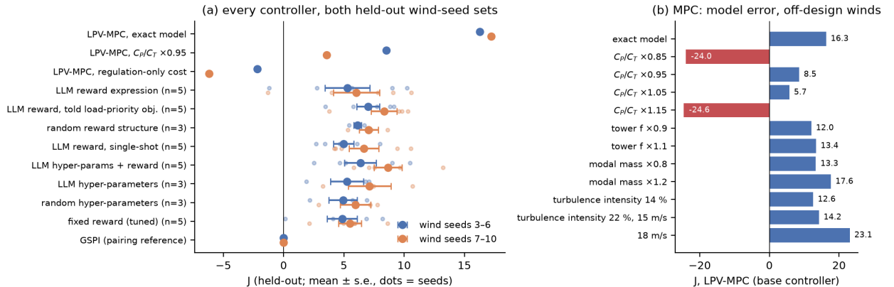
Figure 8: (a) J of every GSPI-base controller and of the MPC (as base controller) on both held-out sets. (b) The MPC under model error and off-design winds (the data of Fig. 6, with the wind classes).
