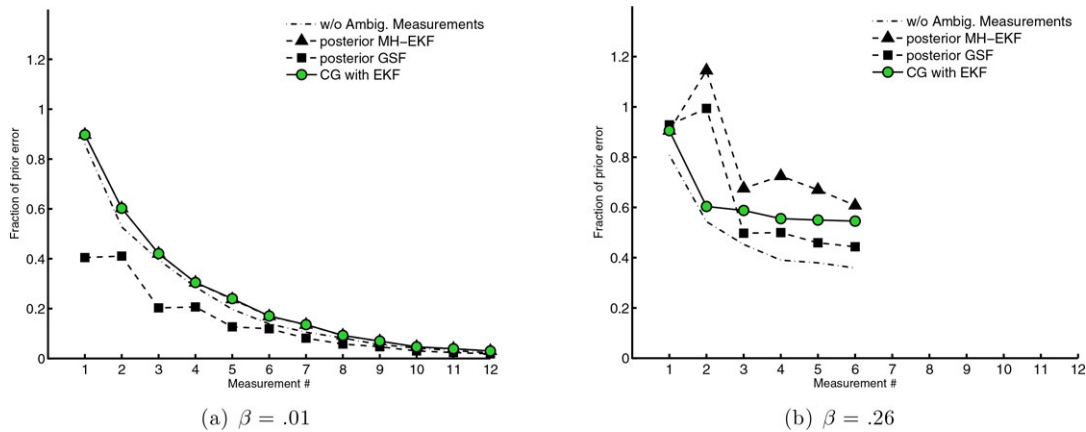
Figure 9. Two examples of the effect of the parameter \beta , comparing the difference in final estimates using an EKF, MH-EKF, and Gaussian sum filter. Shown is the median error over 1,000 trials, after each measurement, for all three filters, as well as an “omniscient” EKF that was given the correct, unambiguous measurements. (a) With \beta = 0.01 , we notice agreement and small final error. (b) With \beta > 0.2 , we notice reduced performance in all filters. These observations suggest that the measurement locations corresponding to low values of \beta are useful for mitigating the effect of ambiguous measurements, as suggested by Lemma 1.
