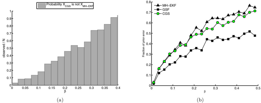
Figure 8. (a) The observed probability that the MH-EKF tracks a different hypothesis than the \beta -Cautious strategy. Note that for small \beta , the \beta -Cautious strategy causes the EKF to track the correct hypothesis more often. (b) The normalized error of the final estimate [\|\hat{x}(n) - x^*\| / \|\hat{x}(0) - x^*\|] as a function of the \beta parameter. The median error is shown for the Gaussian Sum Filter, MH-EKF, and \beta -Cautious strategy using an EKF. Note that increasing \beta results in more error, but at less cost as shown in Figure 10.
