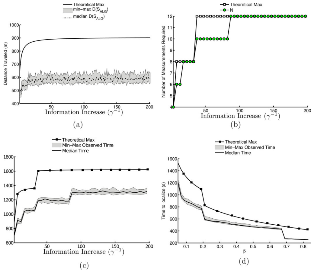
Figure 10. Simulation studies of the possible configurations and the resulting upper bound. We vary the final required uncertainty ( \gamma ) and evaluate the costs as shown in Theorem 1. (a) The distance traveled as \gamma decreases (corresponding to a more precise final estimate). (b) The number of measurements taken. (c) The total execution time as \gamma decreases. Part (d) shows the tradeoff between increasing the parameter \beta and the resulting time required to localize the target. Note that the target can be localized more quickly by increasing risk. The discrete drops in time correspond to removing a measurement from the sequence, and the remaining reduction in time is from placing the measurements closer together. Both will cause more error in the final estimate, as shown in Figure 8(b).
