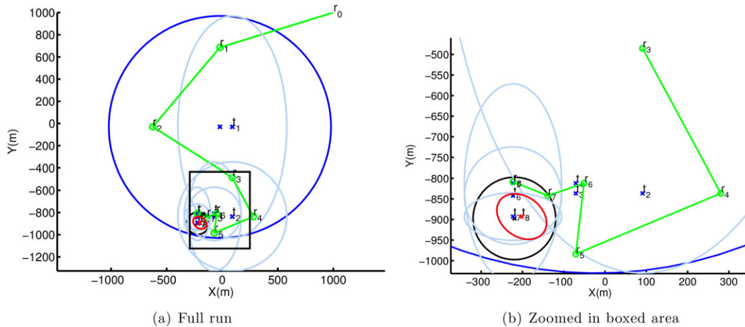
Figure 4. A simulated execution of the cautious strategy. This figure is best viewed in color. (a) The full run. (b) Detail of the boxed region in the first figure. A red ellipse denotes the final target covariance, the black circle is the desired uncertainty, blue is the prior estimate, and green is the robot path and measurement locations. The robot travels in a roughly zigzag path toward the target, while the target hypothesis shifts rectilinearly toward the true target.
