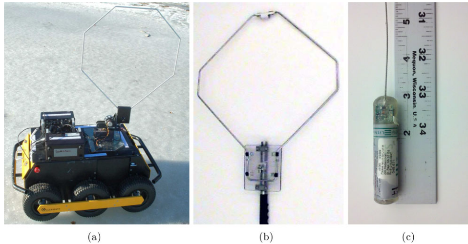
Figure 12. (a) The robotics platform employed in field tests. Notice the octagonal antenna used to detect nearby radio transmitters, and the servomotor used to rotate the antenna. The robot has been tested on multiple lakes in Minnesota, including Lakes Gervais, Staring, Keller, and Phalen. (b) The antenna used to gather bearing measurements. The antenna is radially symmetric, producing ambiguous bearing measurements. The antenna is approximately 56 cm (22 in) in diameter and is mounted on a servomotor attached to the robotic chassis. (c) A radio transmitter that is surgically implanted in invasive fish. Each transmitter (or “tag”) has a unique frequency and transmits an uncoded pulse at approximately 1.1 Hz. The tags are nearly 7.5 cm (3 in.) long.
