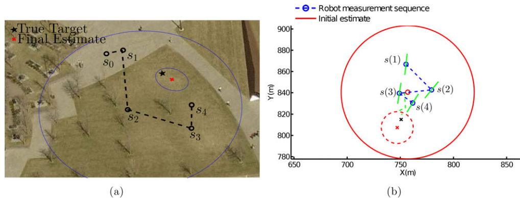
Figure 13. Two single-target field trials. Parameters were \sigma_\beta^2 = 1 and \sigma_s^2 = (\frac{\pi}{8})^2 . In both cases, the time for the system to localize the target adhered to the theoretical bounds. (a) The two \sigma uncertainty ellipses are shown for the prior and final estimates. The final error was less than 5 m after only four measurements. The total experiment area was approximately 70 m by 64 m. (b) At Lake Gervais, MN. With no prior information, the initial estimate was constructed using the routine described in Section 6.2, producing the large red circle shown. The measurement locations narrowed the uncertainty to the final circle given as a dashed line. The true target location is labeled as a black x.
