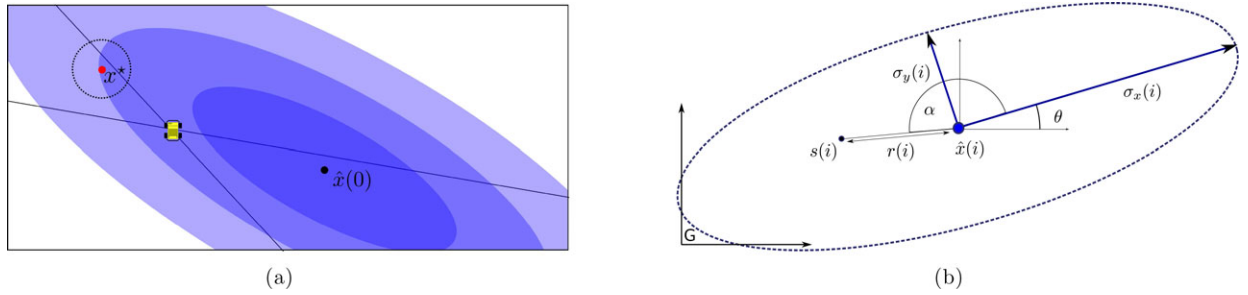
Figure 1. (a) Problem setup. A robot, without knowledge of the true target location x^* but with an initial hypothesis of the target location, \hat{x}(0) , must find measurement locations to shrink the uncertainty about x^* . Measurements taken far from x^* , for example, near \hat{x}(0) , will ultimately provide little information about x^* and are thus wasteful. Shown is an example of a “double wedge” or ambiguous measurement cone: From just one measurement, it is not clear if the target is near \hat{x}(0) or x^* . (b) The notation and problem formulation. A sensor location at time i , denoted s(i) , is described by (r(i), \alpha(i)) . Here r(i) is the range from the sensor to the current hypothesis, \hat{x}(i) , and \alpha(i) denotes the orientation with respect to the line formed by the major axis of the covariance ellipse, \Sigma(i) , with eigenvalues \sigma_x(i) and \sigma_y(i) and orientation \theta(i) with respect to a global frame.
