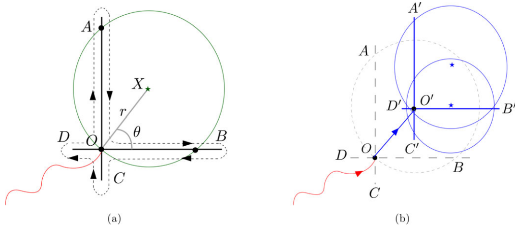
Figure 5. Search-based initialization. (a) The robot continues along an arbitrary but fixed direction until it cannot detect the signal from X (at position A ). The robot then returns to O and repeats the same strategy along a perpendicular line ( B ). In general, the O can lie in the interior of the sensing circle, hence the robot also searches along C and D . (b) A second search from the center of the first circle will reveal all nearby tags, provided the sensing range is larger than the spacing between targets.
