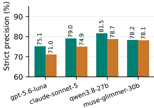
(b) Strict precision P_strict
