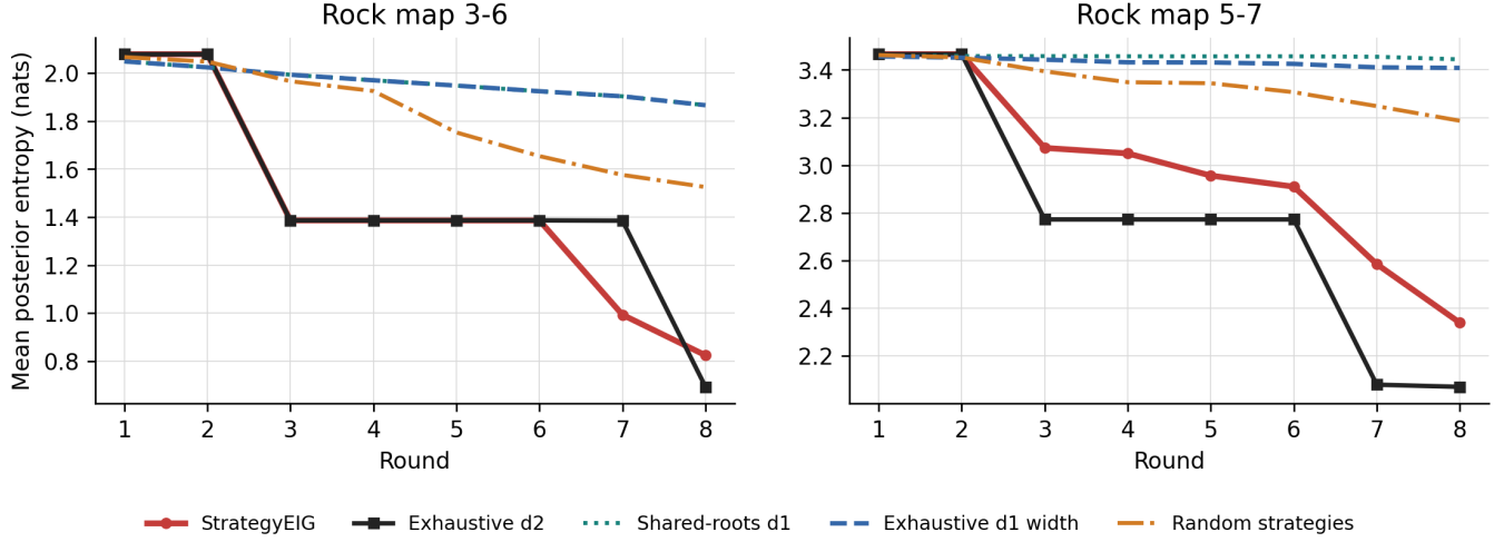
Figure 2: Mean posterior entropy over 30 paired trajectories per map. StrategyEIG and exhaustive d2 first spend zero-information actions on movement, then obtain large entropy drops from more accurate checks.
