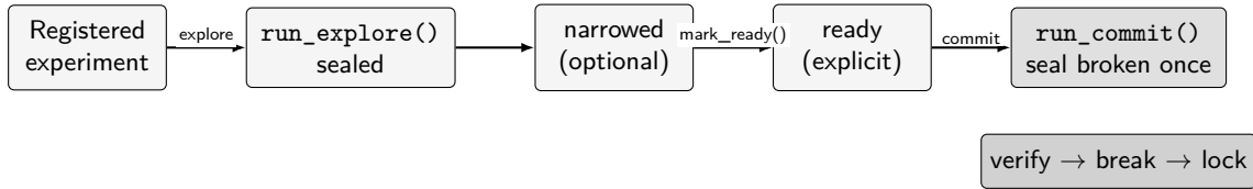
Figure 3: Explore / commit lifecycle for a registered experiment. Only run_commit() (right-most stage) breaks the seal after verify() passes; a broken seal cannot be re-sealed, and re-running run_explore() does not consume the holdout.
