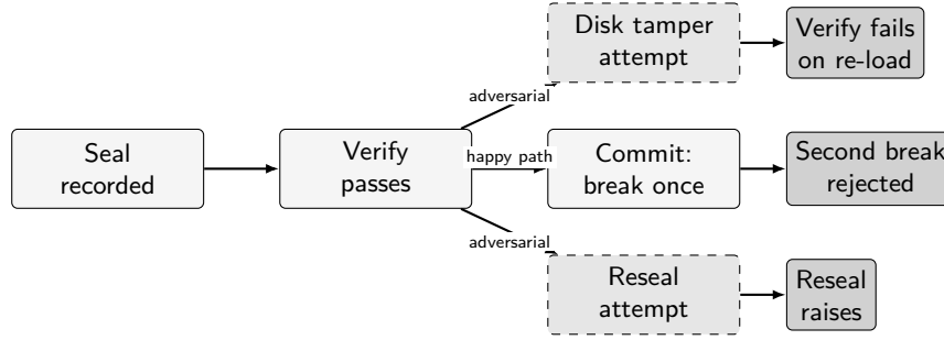
Figure 2: Seal lifecycle paths exercised by scripts/reproduce_seal_demo.py . verify after seal creation returns the canonical-OK state; from there, three audit forks are explored: an on-disk tamper attempt (verify fails), the happy-path commit (single break succeeds, second break is rejected), and a reseal attempt on a still-sealed file (raises). Adversarial forks use a dashed style; success nodes are filled lightly; failure endpoints are darker. The micro-demo uses a temporary seal file and fixed digest; it does not open registered-experiment holdouts or touch data_cache/ .
