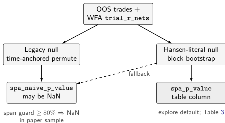
Figure 4: Dual-null SPA wiring on the explore path. Both p -values are stored; Table 3 reports Hansen-path spa_p_value . Legacy NaN under the anchor-span guard is intentional, not a failed run.
