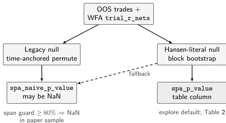
Figure 3: Dual-null SPA wiring on the explore path. Both p -values are stored; Table 2 reports Hansen-path spa_p_value . Legacy NaN under the anchor-span guard is intentional, not a failed run.
