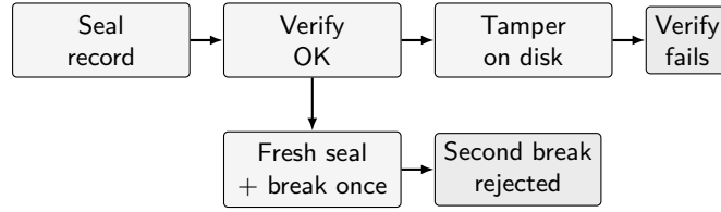
Figure 2: Synthetic Claim 1 micro-demo path ( scripts/reproduce_seal_demo.py ). The demo uses a temporary seal file and fixed digest; it does not open registered-experiment holdouts or touch data_cache/ .
