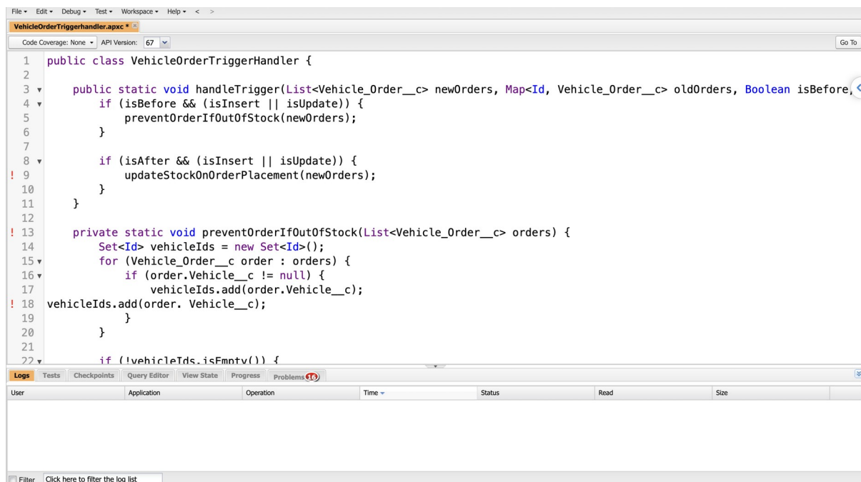
Figure 19 VehicleOrderTriggerHandler class in Developer Console
