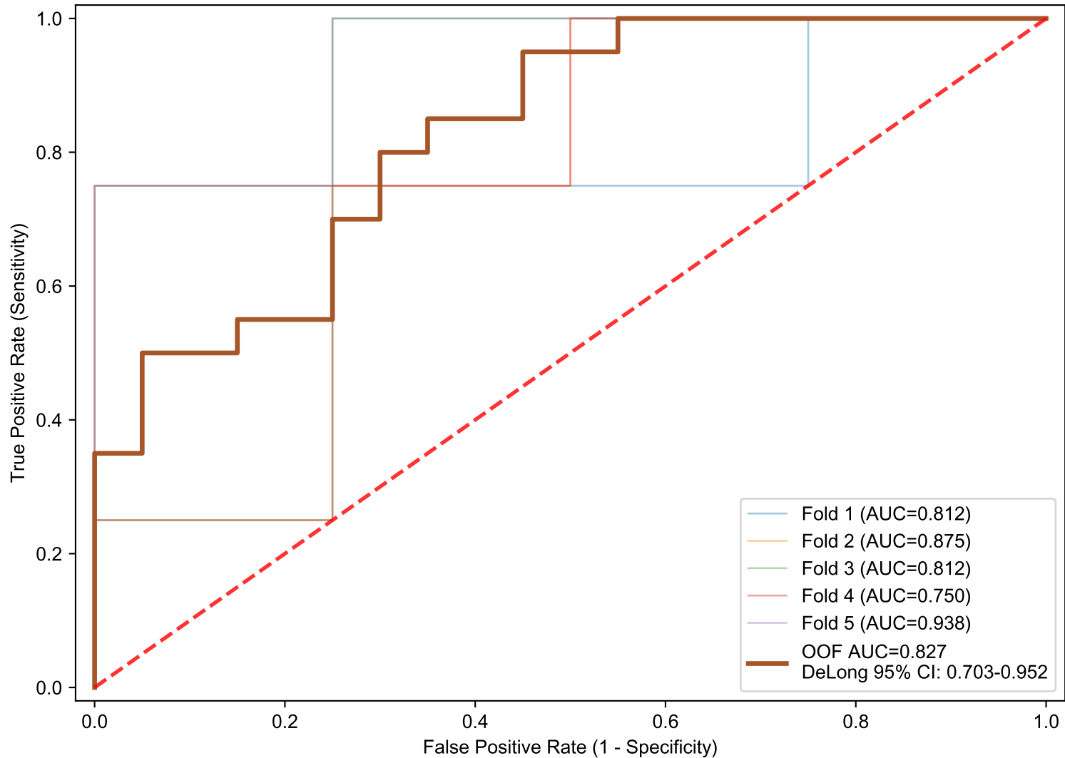
GLM ROC Curves (5-Fold CV)
